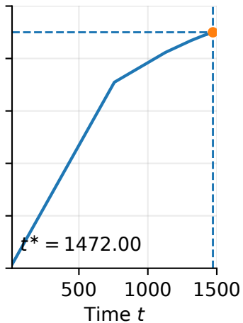
Representative fidelity traces for n = 5 \rho = 10
