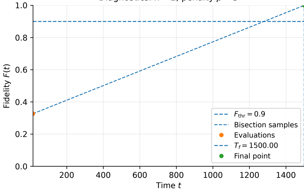
Diagnostics: n = 2 , penalty p = 5
