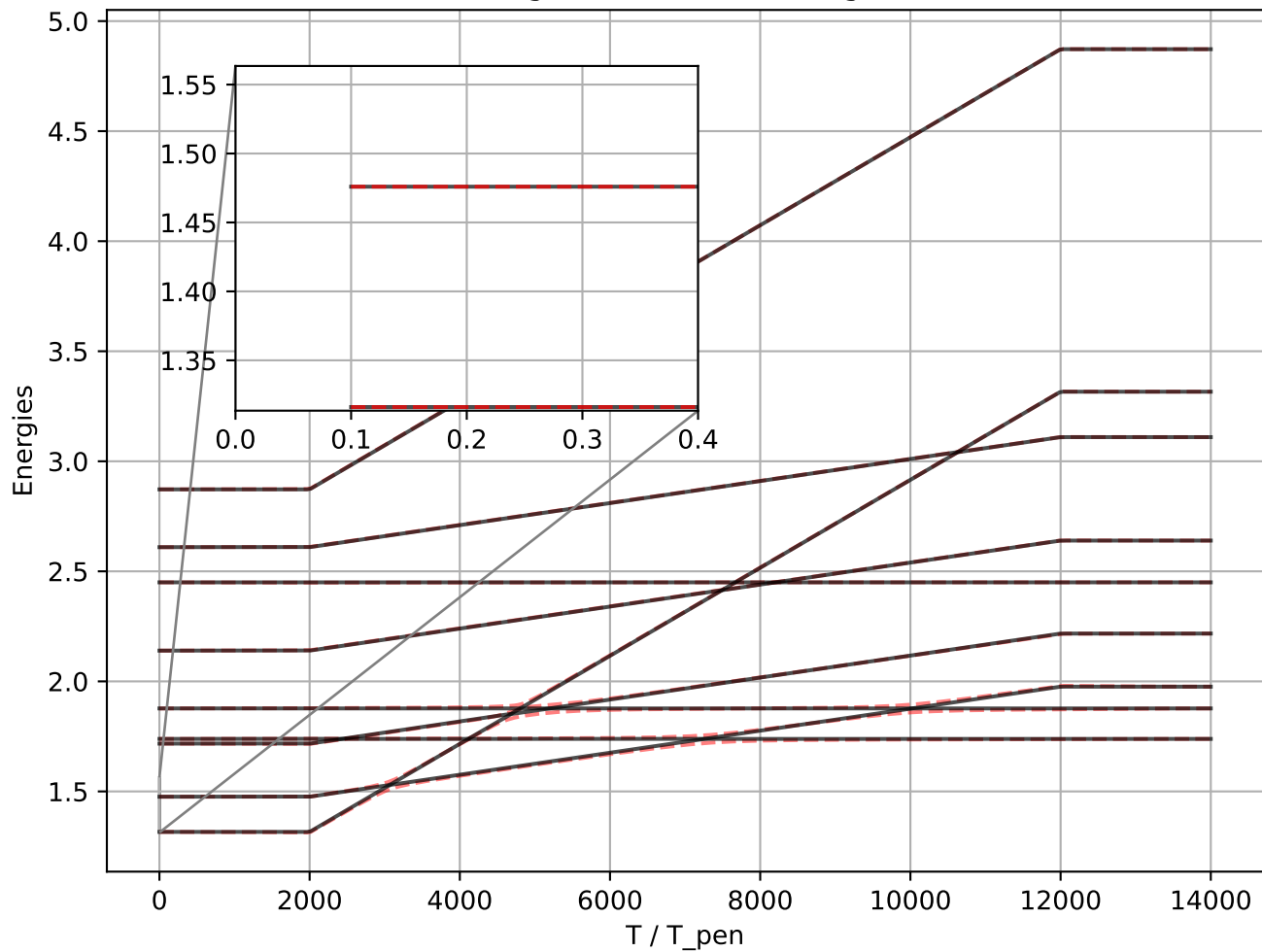
Avoided crossings (black) vs crossings (red dashed)
