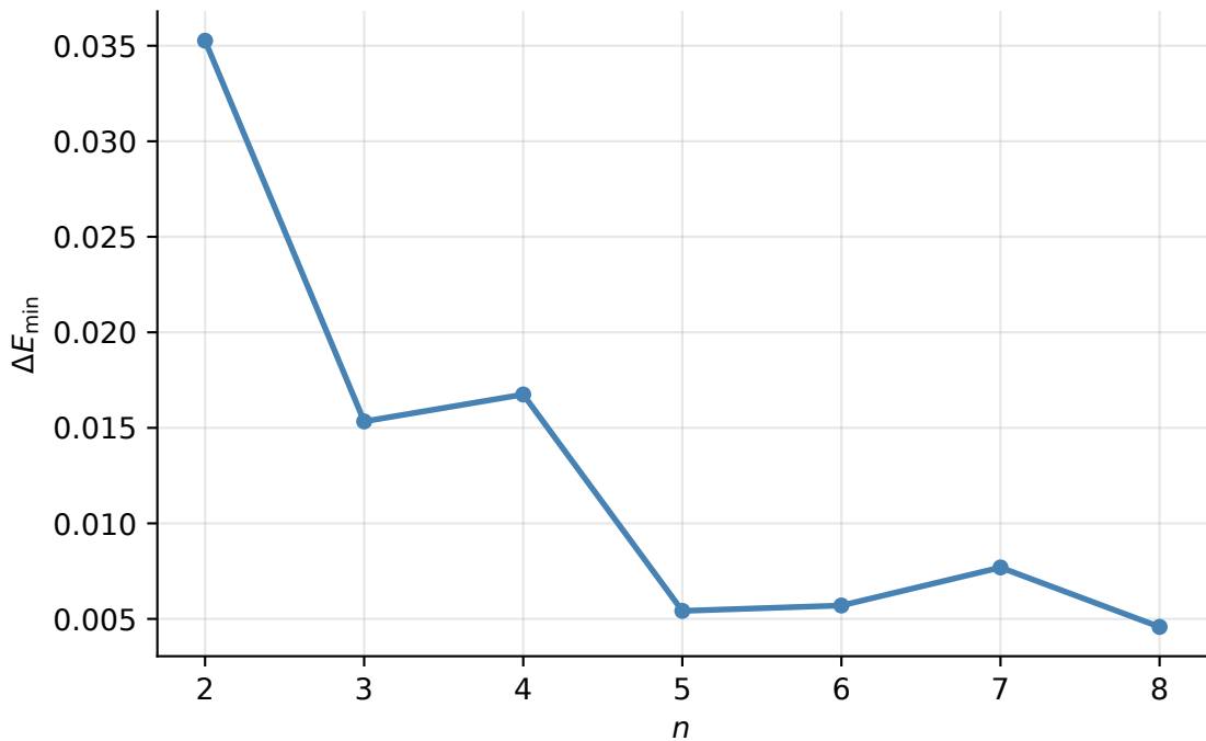
Minimal energy gap vs n
