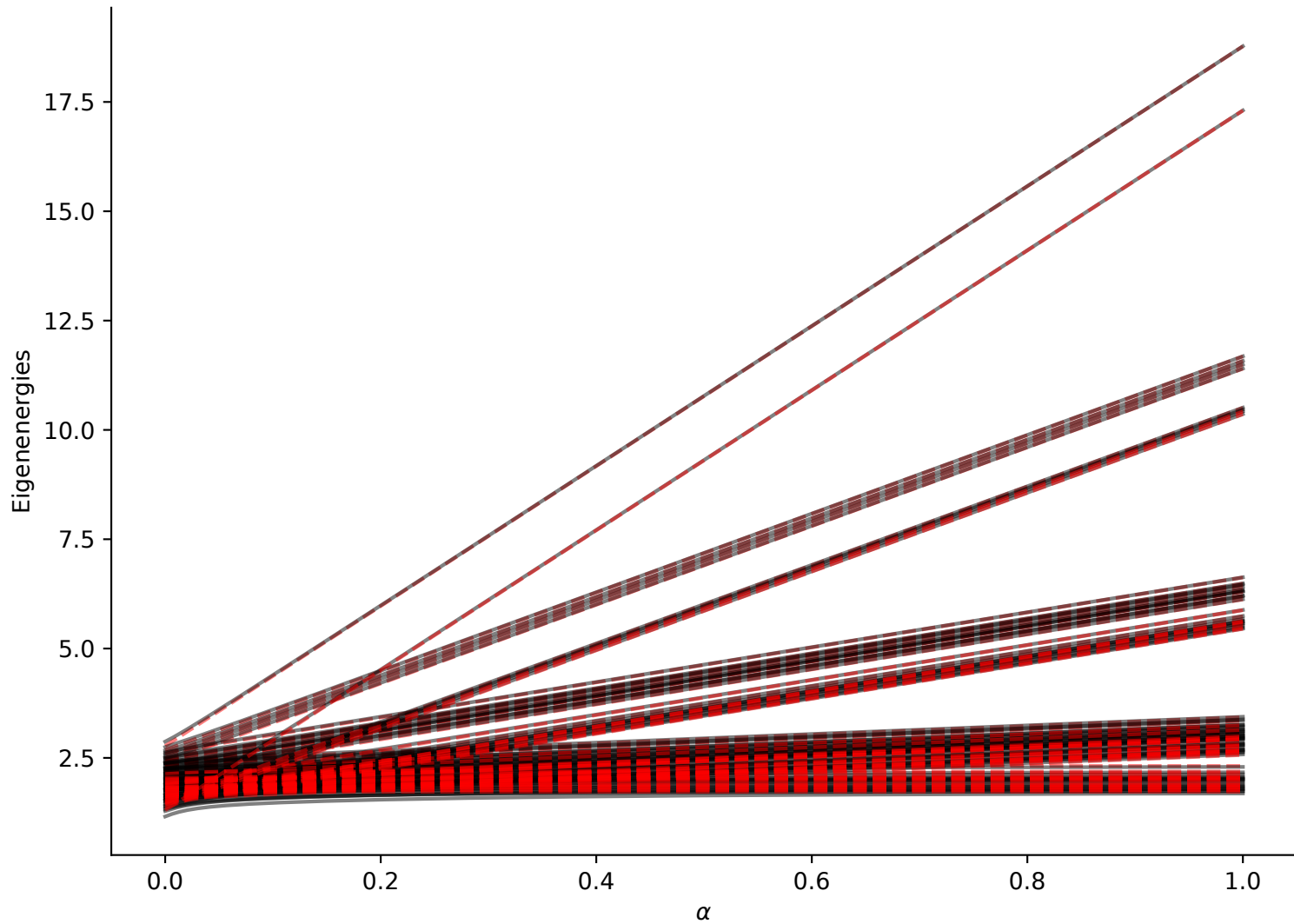
Avoided crossings (black) vs crossings (red dashed)
