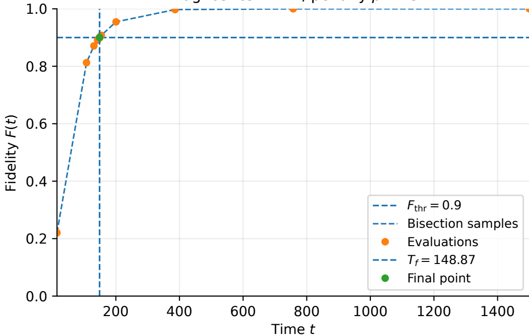
Diagnostics: n = 2 , penalty p = 15
