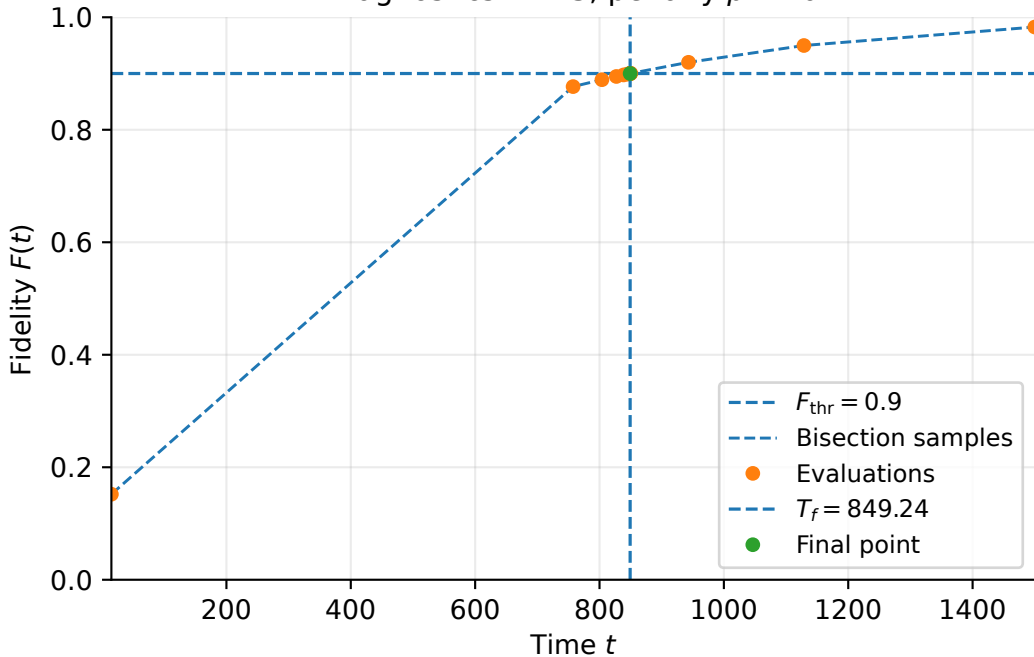
Diagnostics: n = 3 , penalty p = 10
