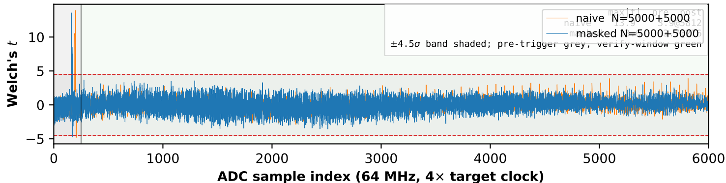
ML-KEM-1024 verify-window 1st-order TVLA, N=5000+5000
