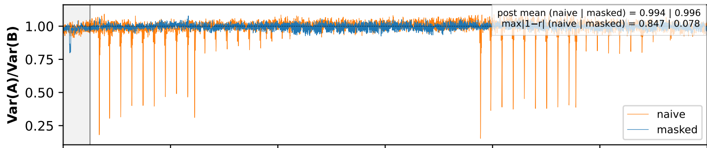
ML-KEM-1024 share-recombine 2nd-order TVLA, naive N=5k vs masked N=10k (ISO 17825)
