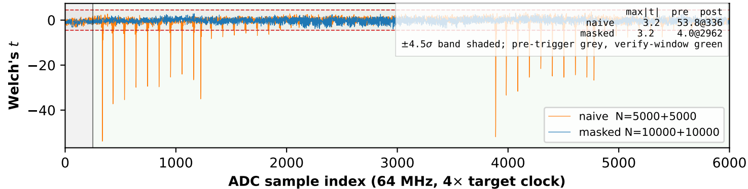
ML-KEM-1024 share-recombine 2nd-order TVLA, naive N=5k vs masked N=10k (ISO 17825)
