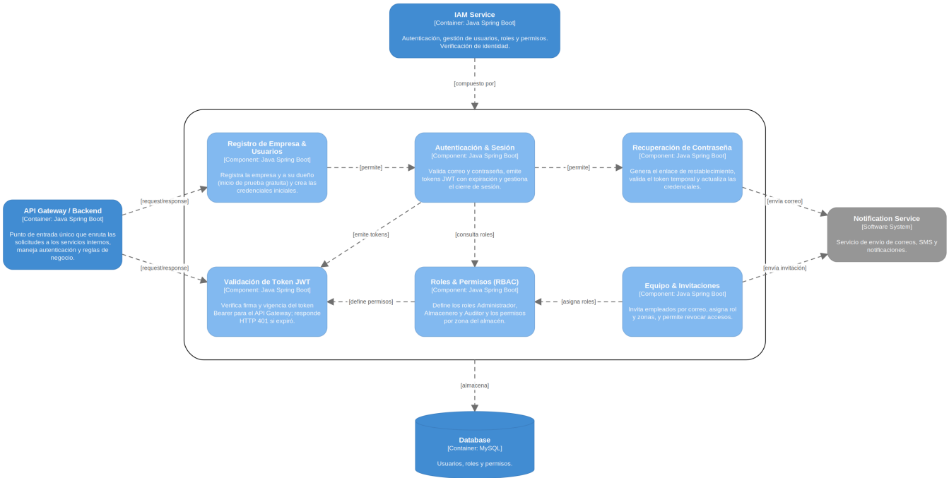
Component Diagram — IAM Service NodeSecure · SafeZone — C4 Nivel 3 (Componentes)
