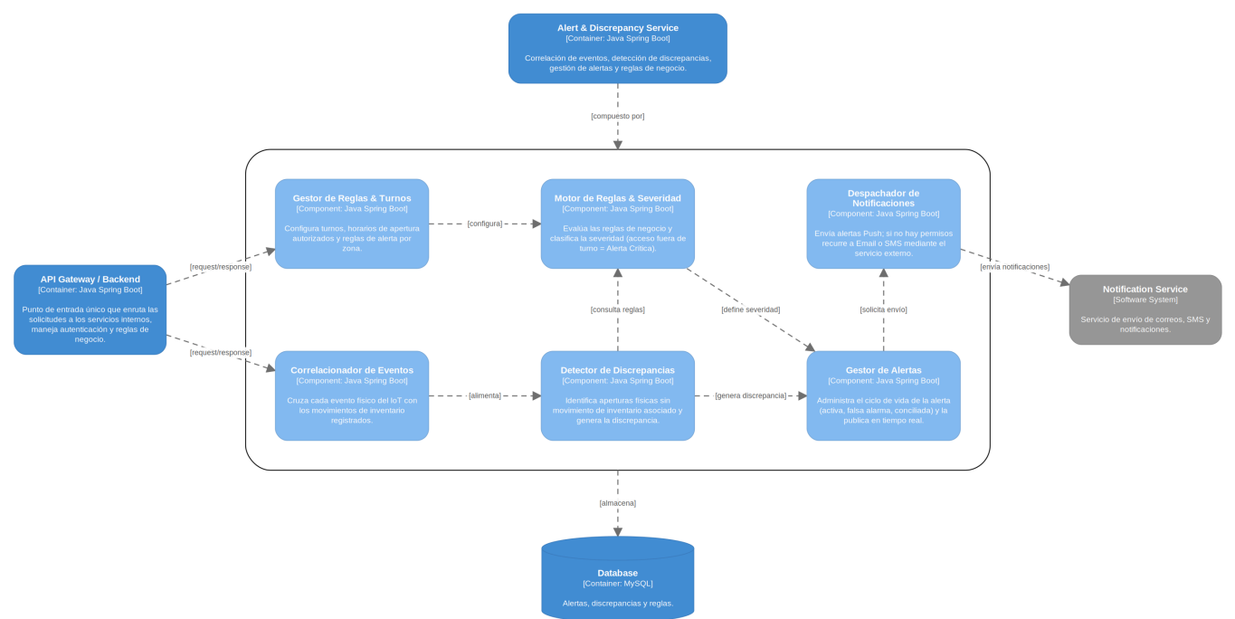
Component Diagram — Alert & Discrepancy Service
