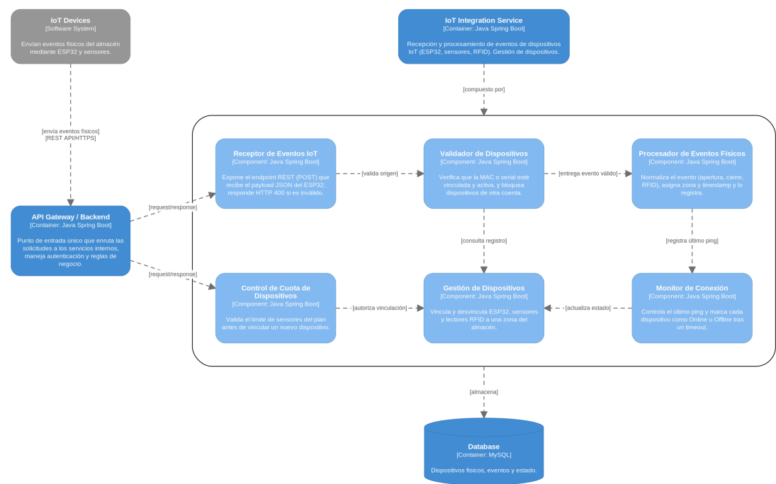
Component Diagram — IoT Integration Service
