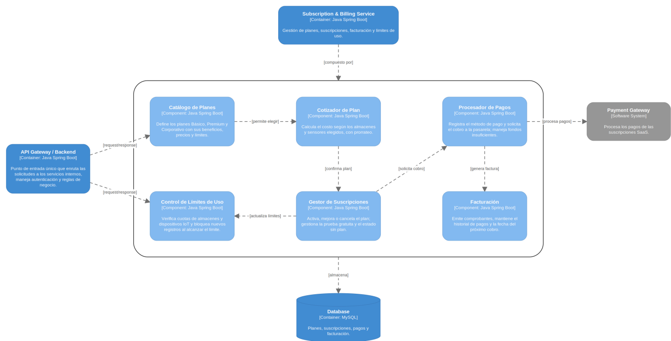
Component Diagram — Subscription & Billing Service NodeSecure - SafeZone — C4 Nivel 3 (Componentes)
