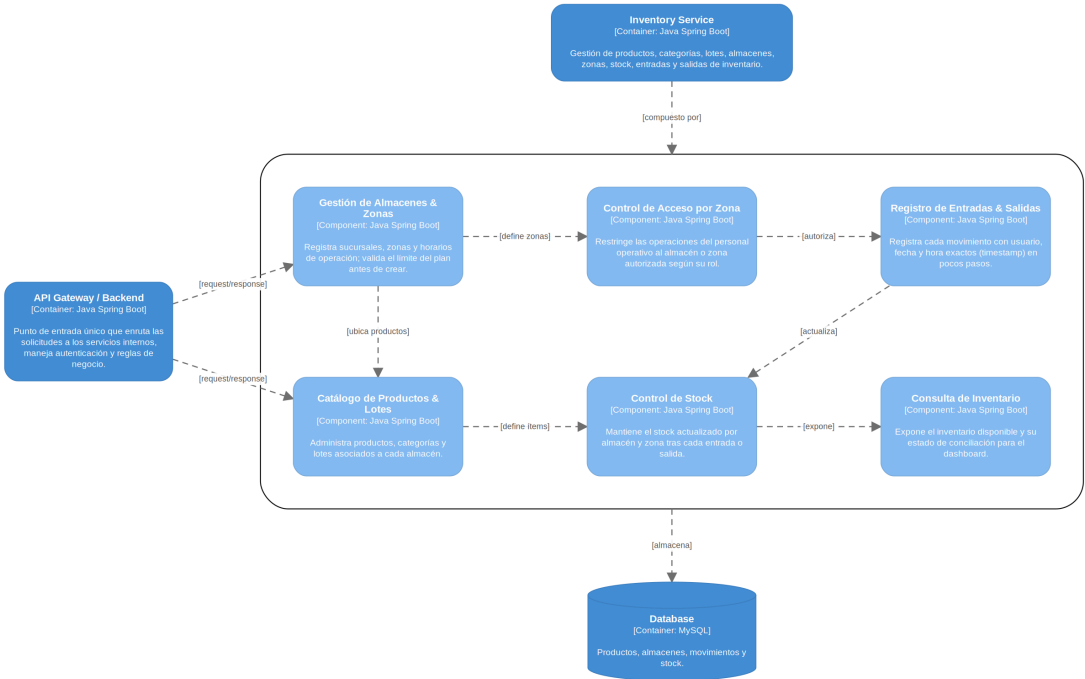
Component Diagram — Inventory Service NodeSecure · SafeZone — C4 Nivel 3 (Componentes)
