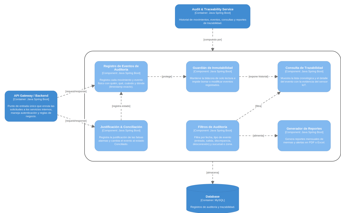
Component Diagram — Audit & Traceability Service
