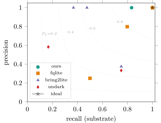
Figure 1: Substrate precision–recall across categories OC/OD/OE with constant- F_1 contours (SQL-DRP omitted: it matches no answer-key row under the format-stable identity). In this harness our carver lies on precision 1.000 in each category.
