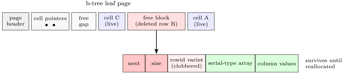
Figure 1: Free blocks (categories 0C/0D) . A deleted row is unlinked from the cell-pointer array; with secure_delete off its bytes remain as a free block inside the still-live leaf page. The 4-byte free-block header overwrites only the leading payload-length and rowid variants—the serial-type array and column values (green) survive in the tail and are reconstructible until the gap is reallocated.
