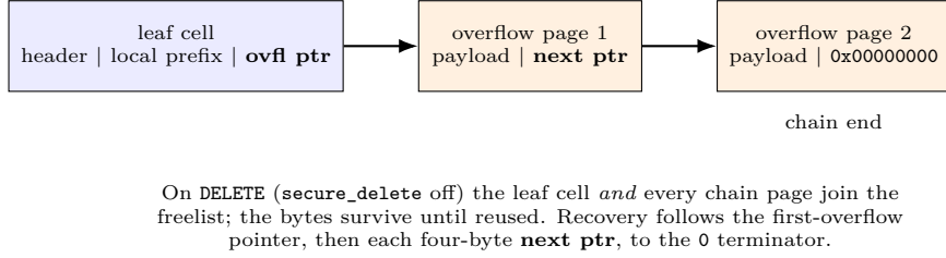
Figure 2: Overflow chains (category 0E) . A value too large for one page spills across a linked chain of overflow pages. A deleted long TEXT/BLOB leaves residue spread over several pages, recoverable only by following the chain through the freelist—and lost once any chain page is reallocated. (In our corpus most 0E bodies were overwritten, so end-to-end 0E recall is 0.333 despite full substrate recall.)
