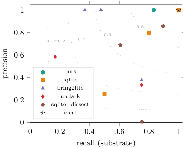
Figure 4: Substrate precision-recall across categories OC/OD/OE with constant- F_1 contours. In this harness our carver lies on precision 1.000 in each category.
