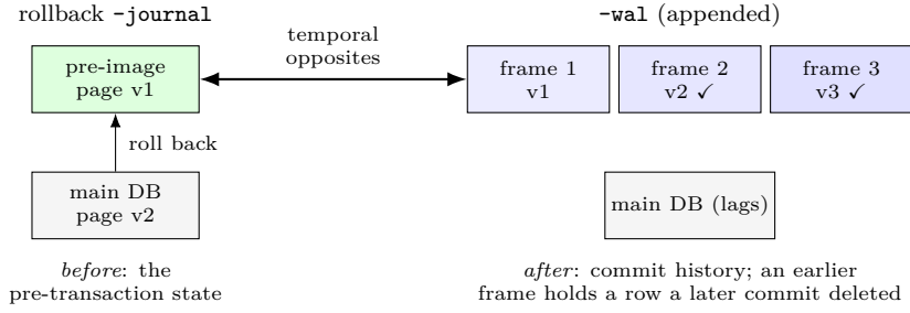
Figure 3: Side files: rollback journal vs. WAL. The two crash-recovery files are temporal opposites. The -journal stores the before -image of each page a transaction will modify (the pre-transaction state). The -wal instead appends new page versions (✓ marks a commit frame) and only later checkpoints them back, so it preserves a multi-commit history in which a row deleted by a later commit still survives in an earlier frame.
