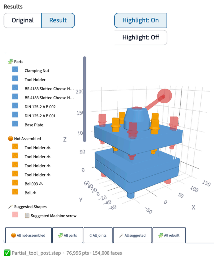
Figure 7.7: Result view of the partial tool post: Parts (blue), Not Assembled (orange) and the Suggested Shapes group (pink).
