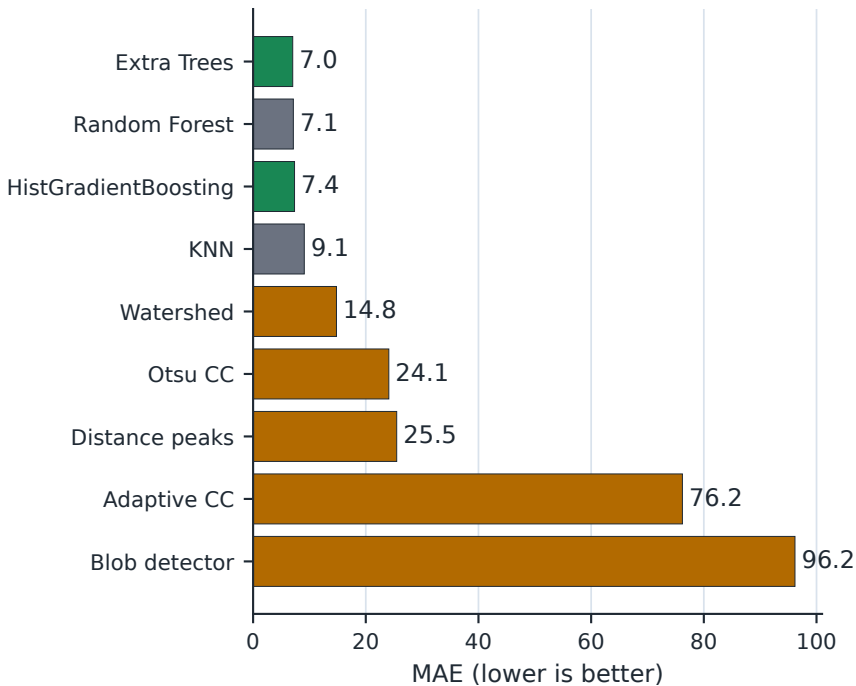
Classical counting baseline MAE
