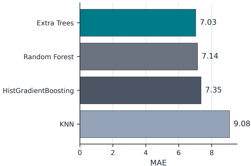
Top classical regressor MAE
