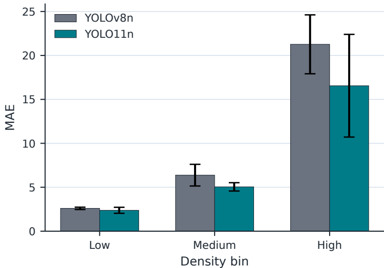
Counting error by density
