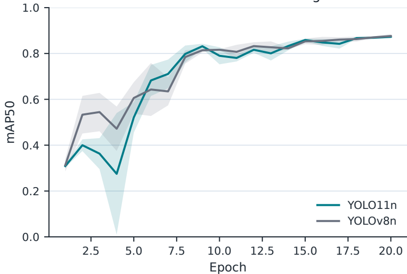
YOLO validation mAP50 convergence
