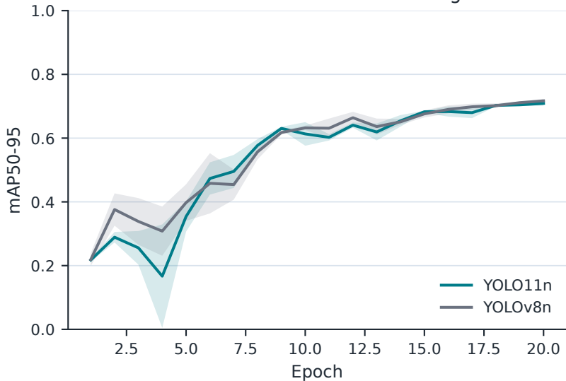
YOLO validation mAP50-95 convergence
