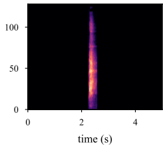
mel band
