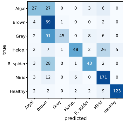
(b) full-integer INT8 (macro-F1 0.6334)
