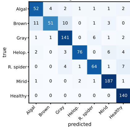
(a) MobileNetV3-Large, FP32 (macro-F1 0.8745)
