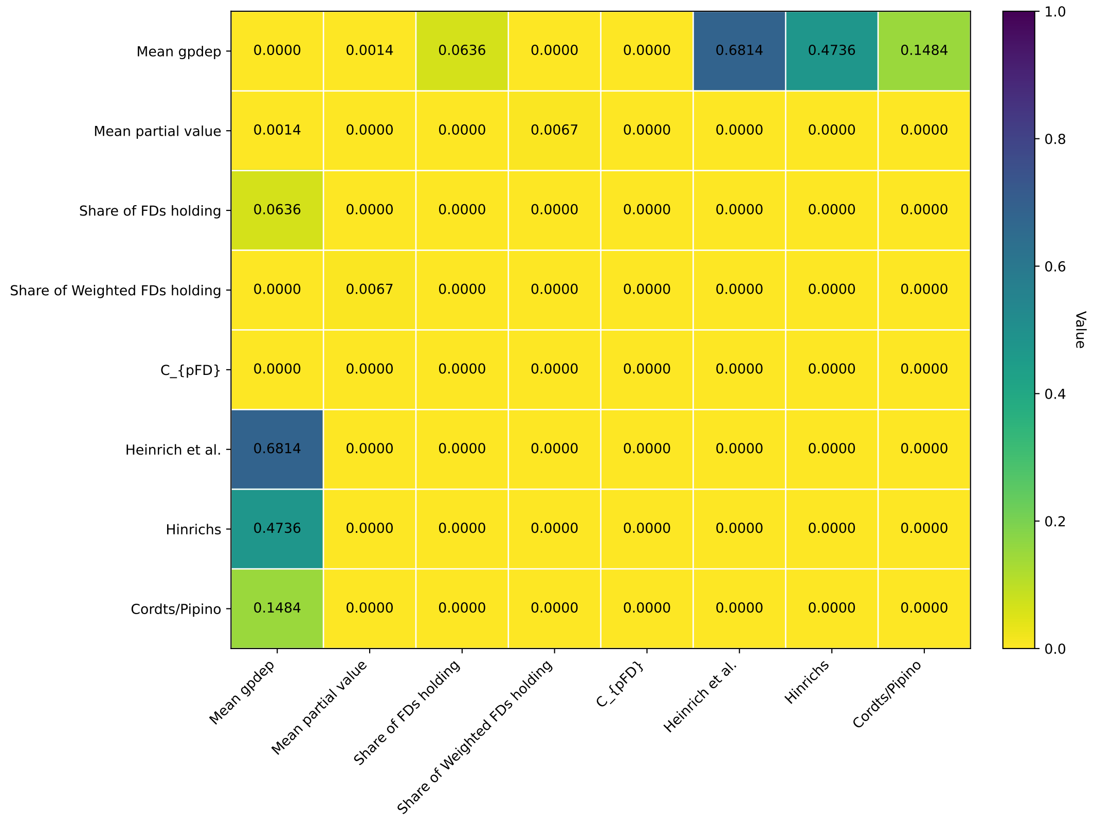
P-value matrix for Pearson correlations
