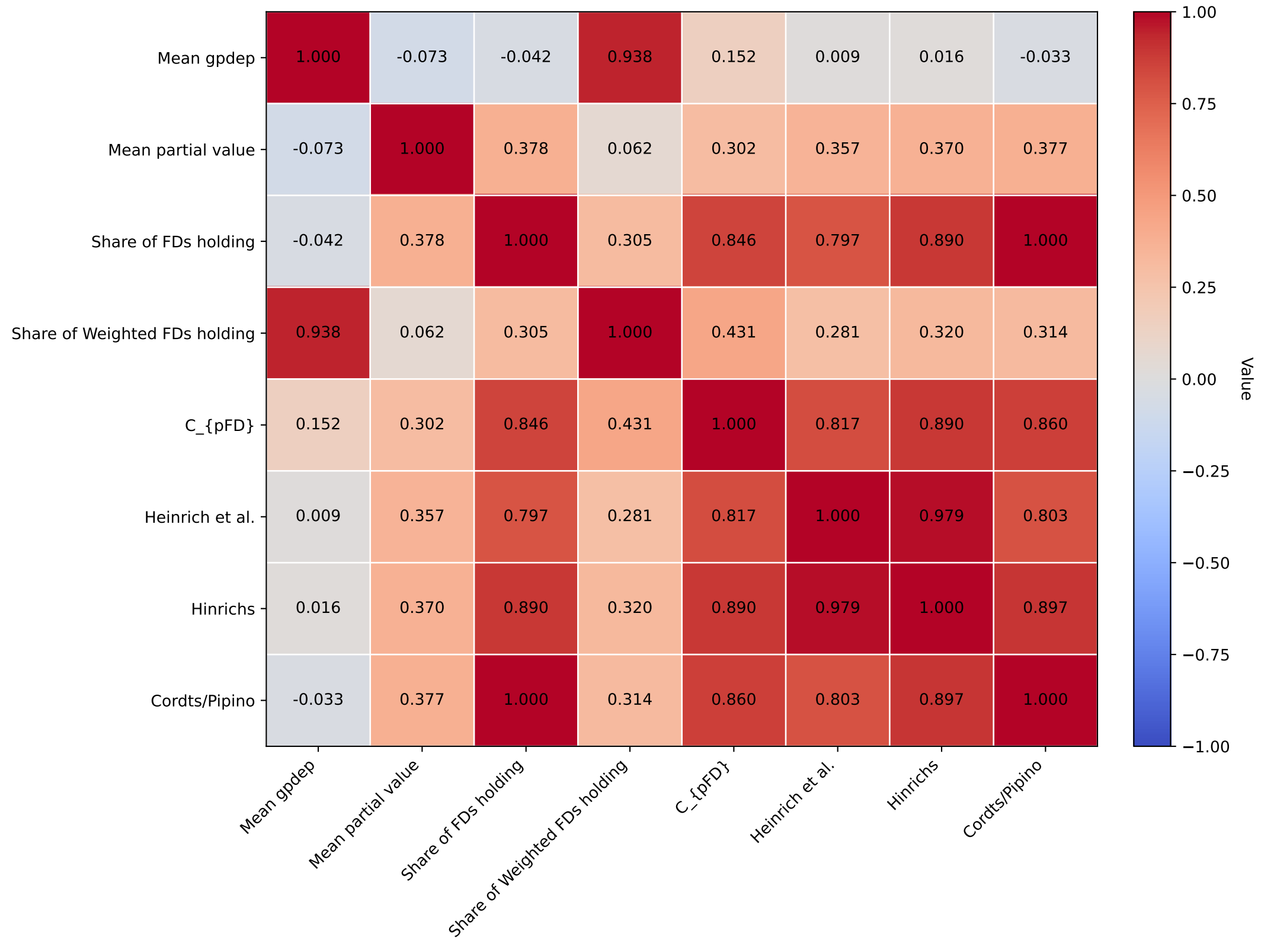
Pearson correlation matrix between dataset-level metrics
