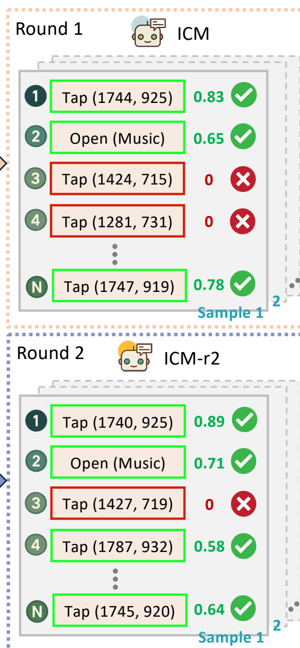
(b) Test-Time scaling pipeline.
