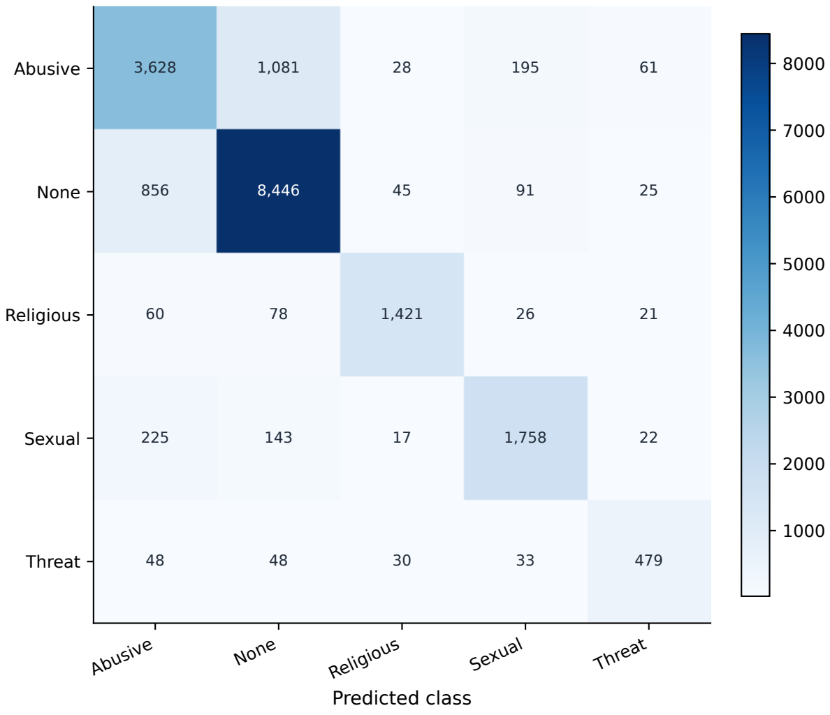
True class
