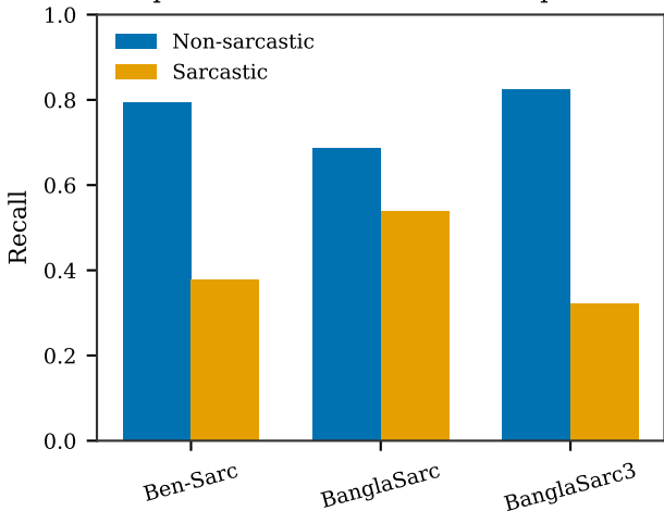
Class-specific recall under cross-corpus transfer
