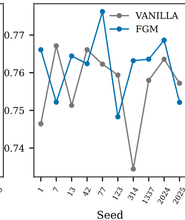
BanglaSarc3
