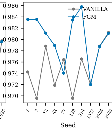
BanglaSarc
