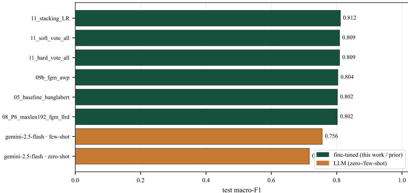
Ben-Sarc (bin) — fitted models vs LLM prompting
