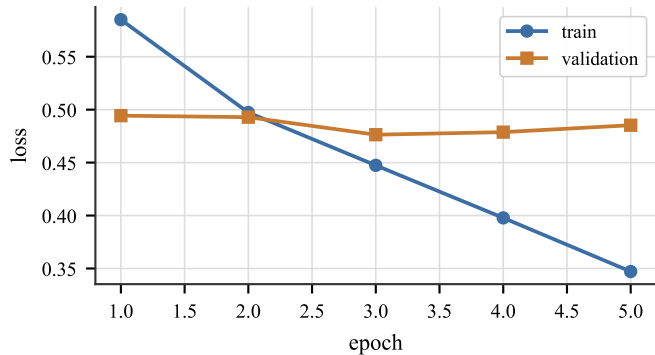
Loss
