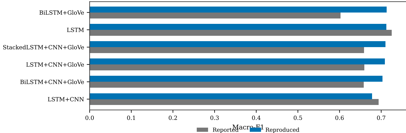
Deep-model reproduction fidelity on the common split
