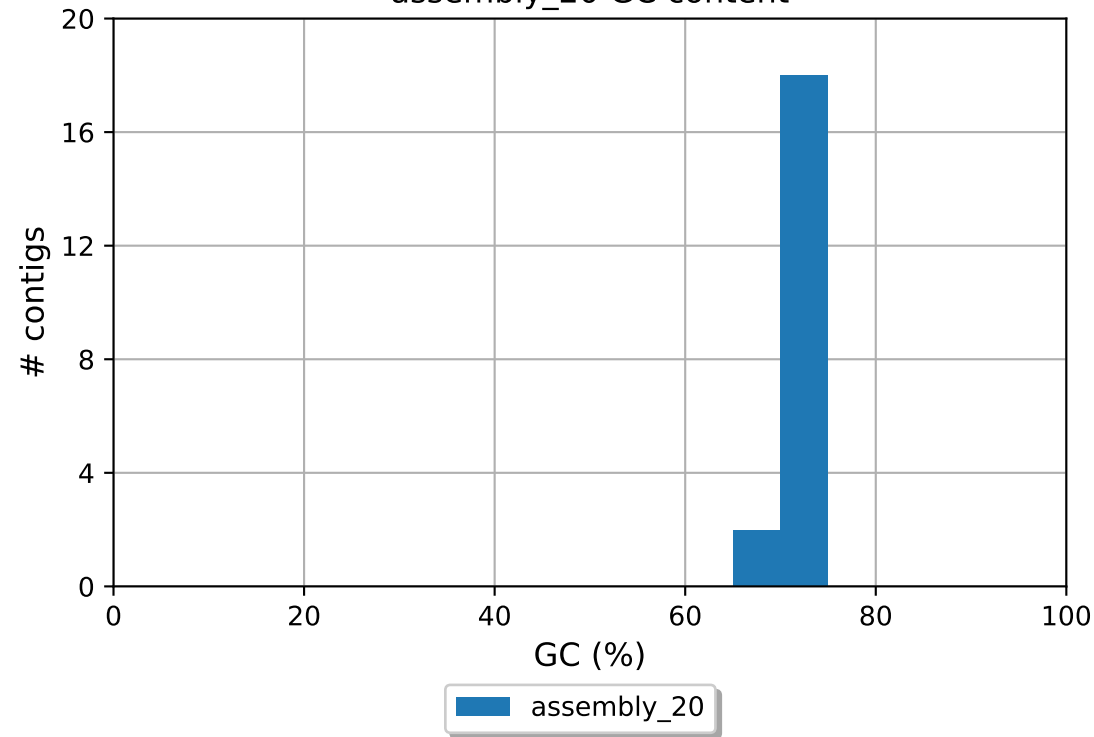
assembly_20 GC content
