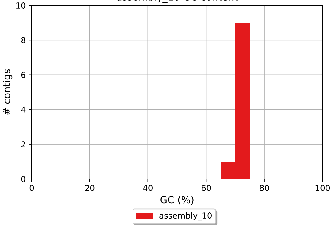
assembly_10 GC content
