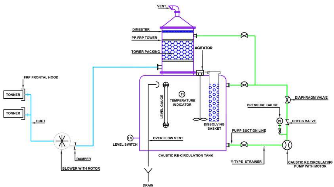
LEAK ABSORPTION SYSTEM
