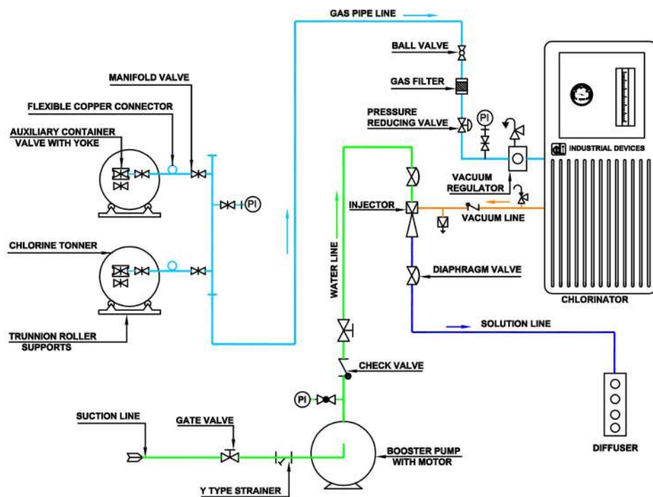
CHLORINATION SYSTEM WITHOUT EVAPORATOR
