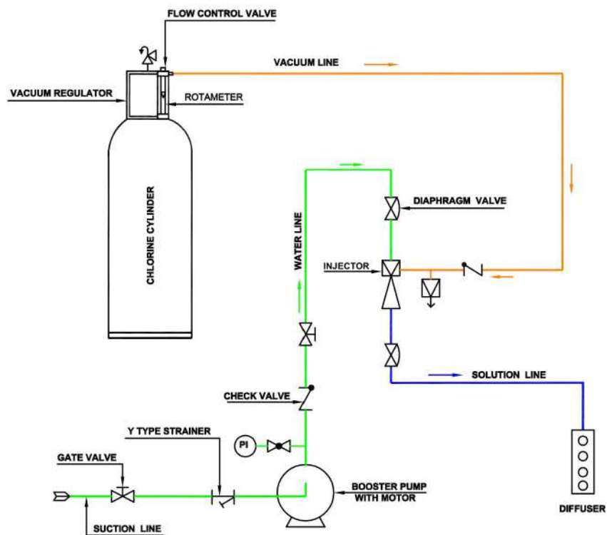
CYLINDER MOUNTED CHLORINATION SYSTEM
