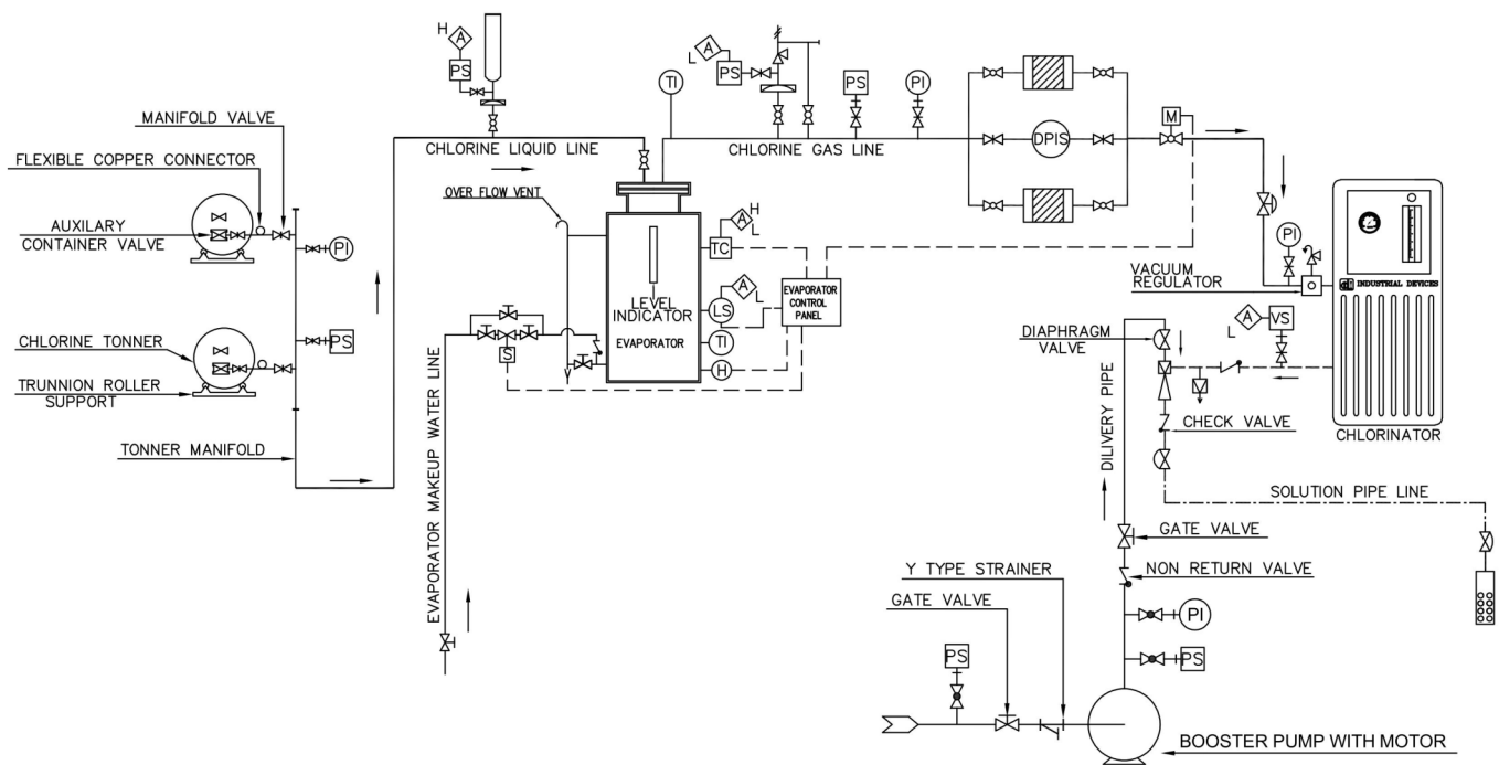
CHLORINATION SYSTEM WITH EVAPORATOR
