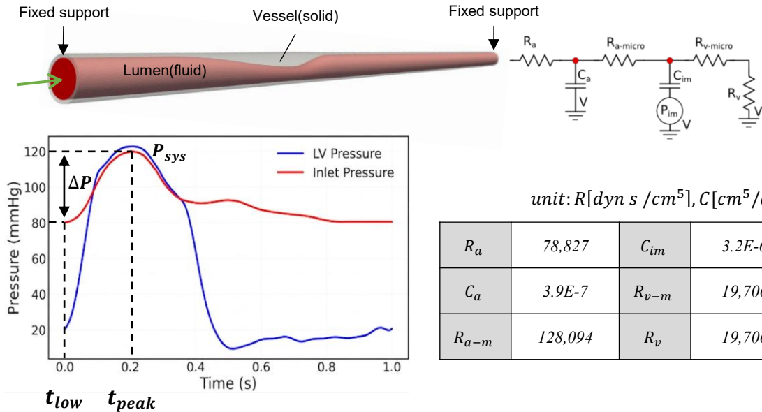
(a) Inlet and Left Ventricular pressure
