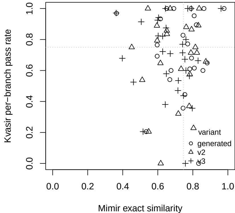
Joint scatter – codex
