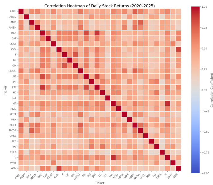
Figure 5.1: Correlation Heatmap of Daily Stock Returns (2020 to 2025)
