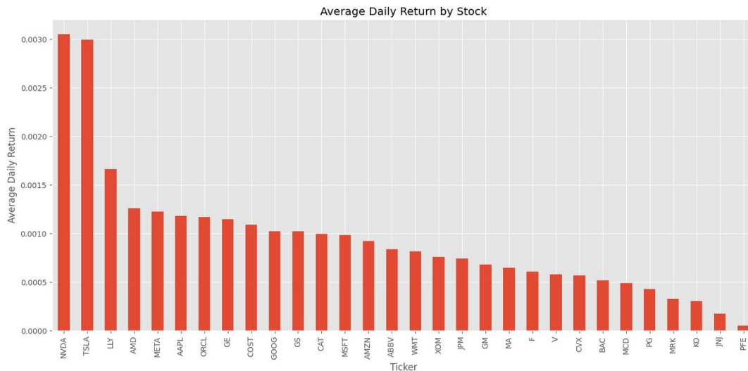
Figure 5.2: Average Daily Return by Stock
