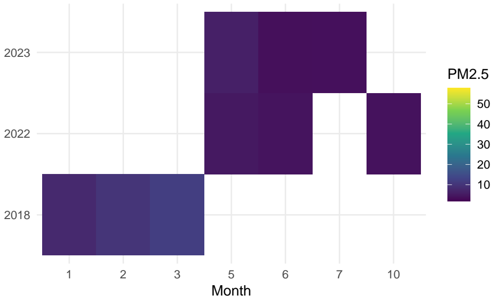
PM2.5 by Month and Year
