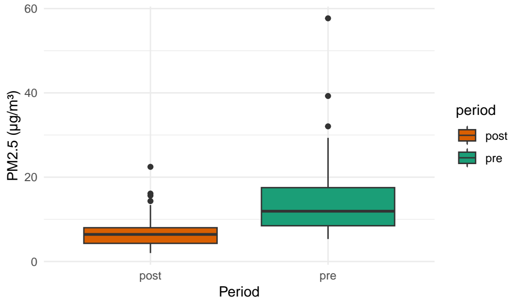
PM2.5 Levels: Pre vs Post COVID
