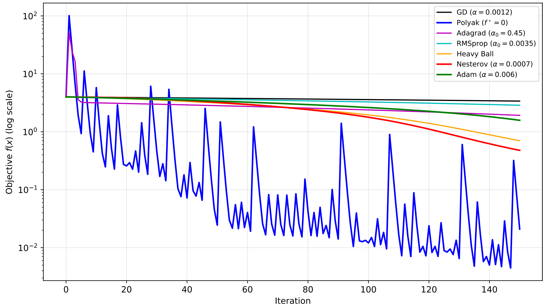
All Methods on Benchmark C (Rosenbrock) — 150 Iterations
