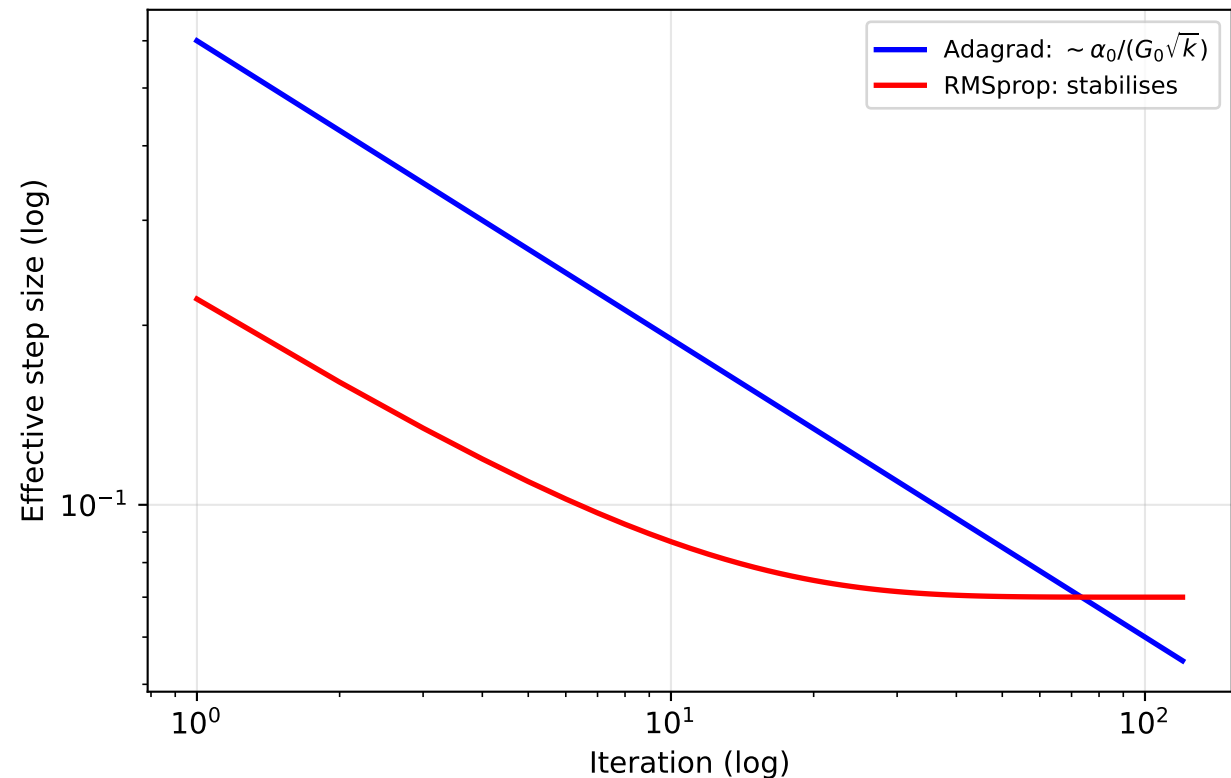
Log-log: Adagrad Decays as O(1/\sqrt{k}) , RMSprop Stabilises
