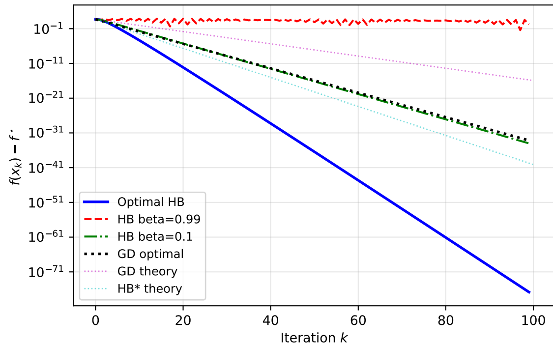
Heavy Ball: Optimal vs Suboptimal ( \kappa = 5 )
