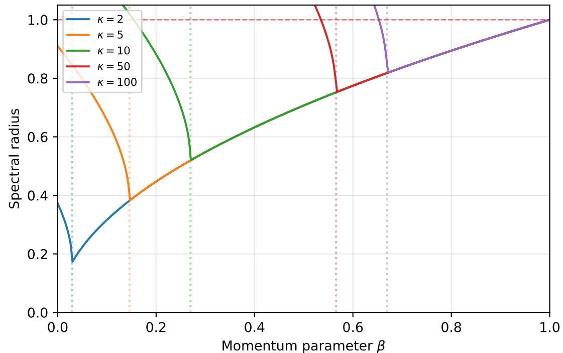
Convergence Rate vs \beta for Different \kappa
