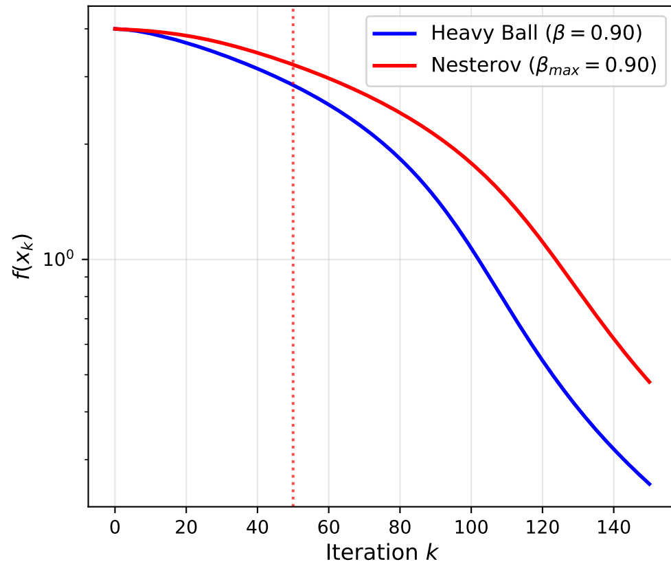
Heavy Ball vs. Nesterov (Benchmark C, Rosenbrock)
