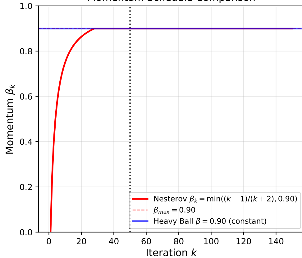
Momentum Schedule Comparison
