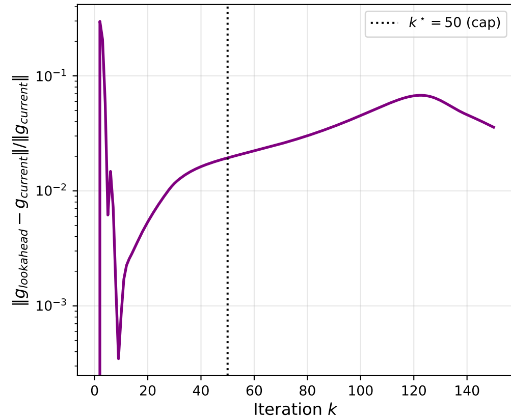
Nesterov Lookahead: Gradient Difference (relative) vs Iteration
