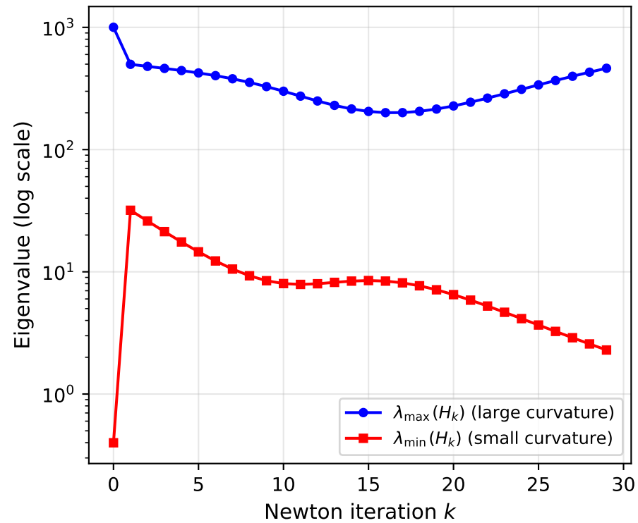
Rosenbrock Hessian Eigenvalues along Newton Trajectory
