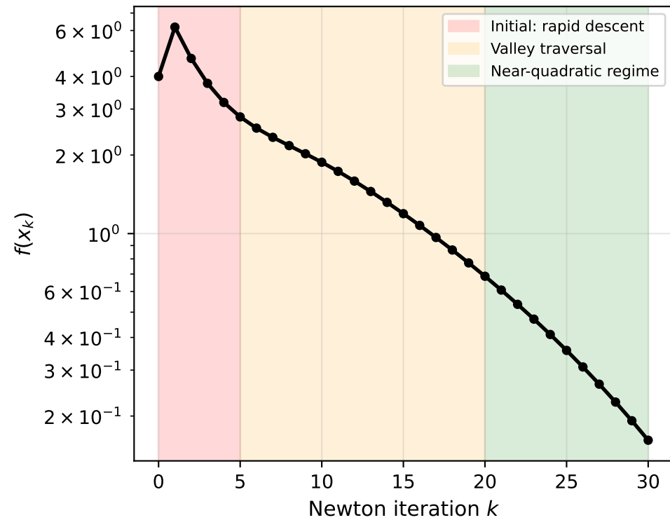
Newton Convergence on Rosenbrock (3 phases annotated)
