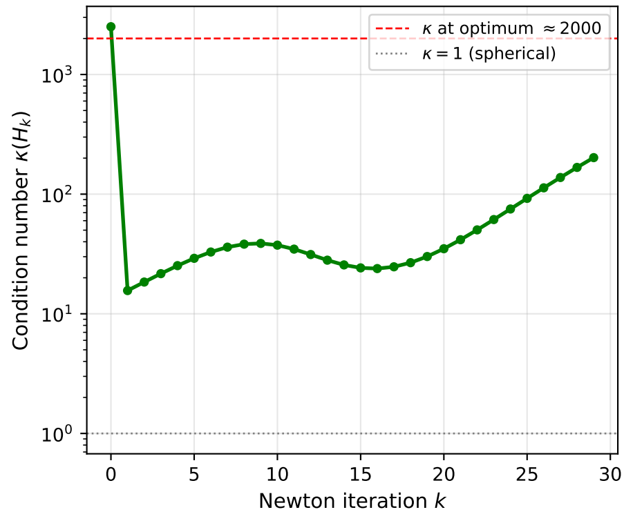
Hessian Condition Number along Newton Trajectory
