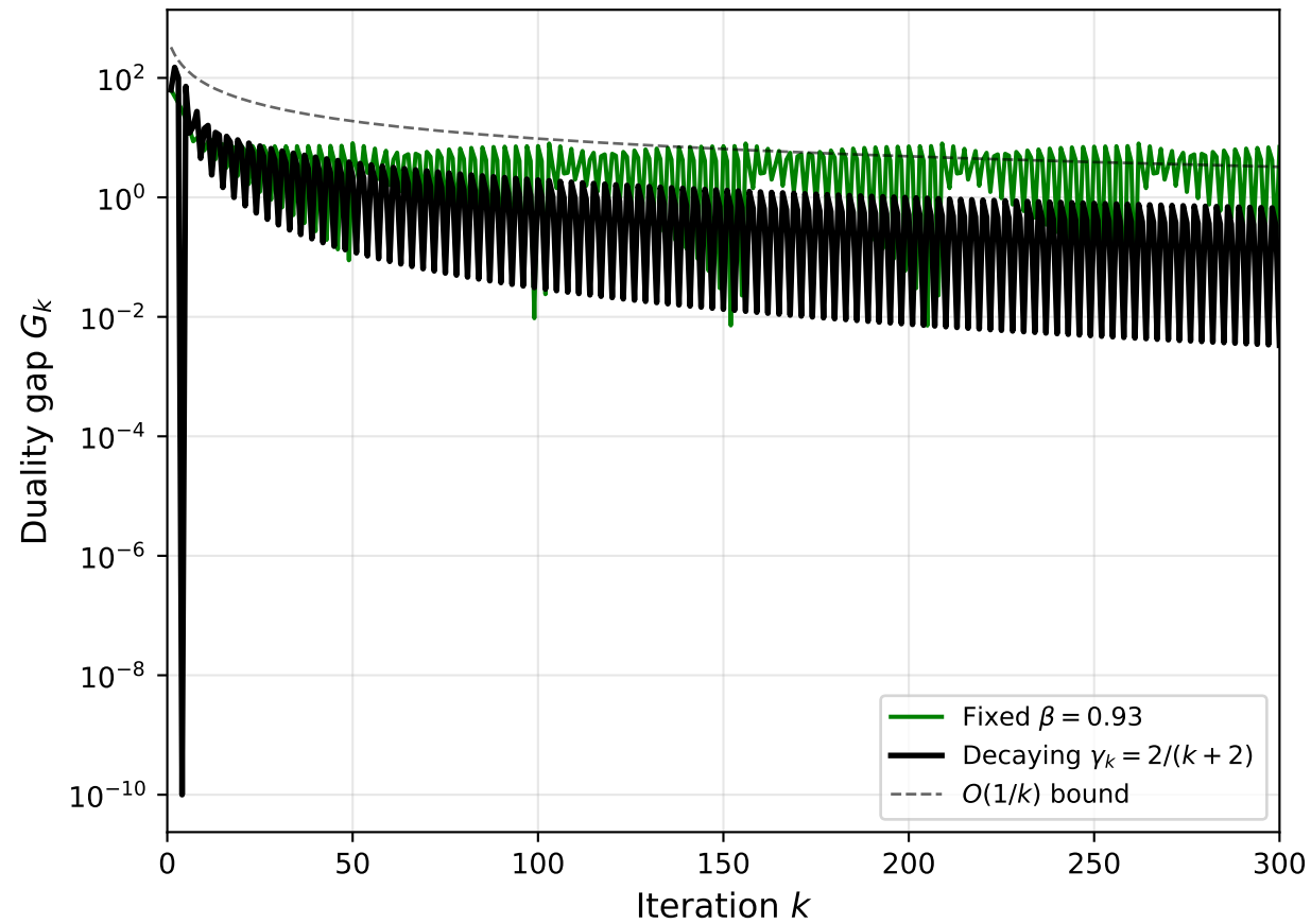
FW Duality Gap: Boundary Optimum (0.5, 0)
