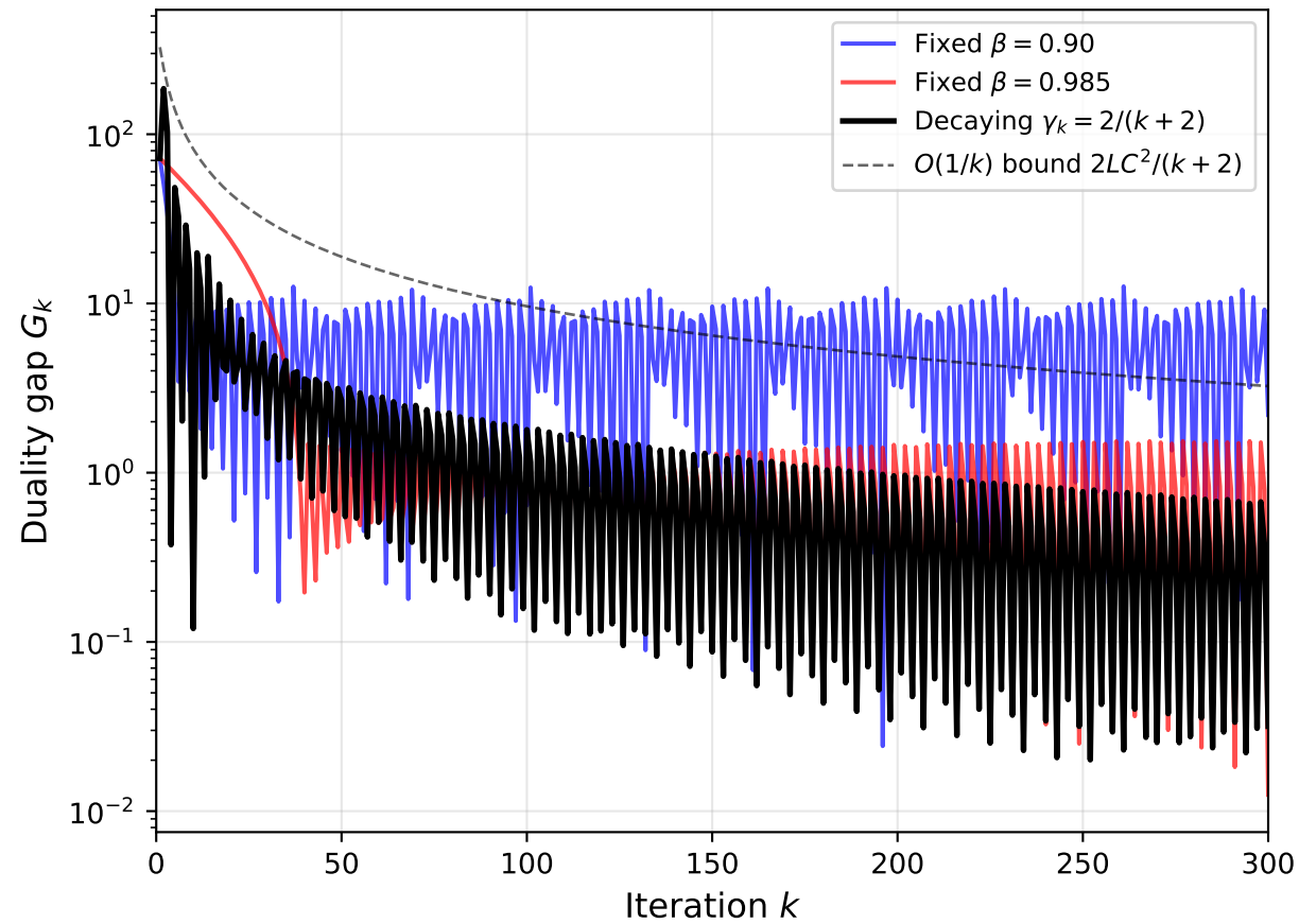
FW Duality Gap: Interior Optimum (1, 5)
