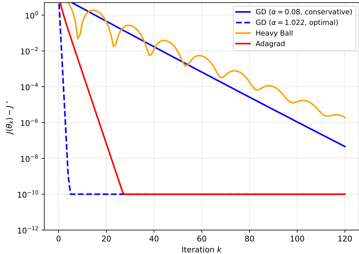
Effect of GD Step Size (Benchmark A, \kappa \approx 1.12 )
