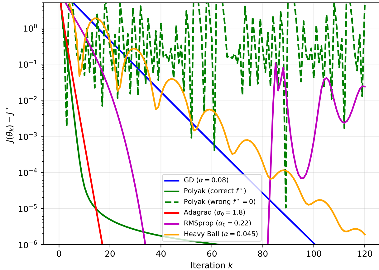
Q1 Methods: Suboptimality on Benchmark A
