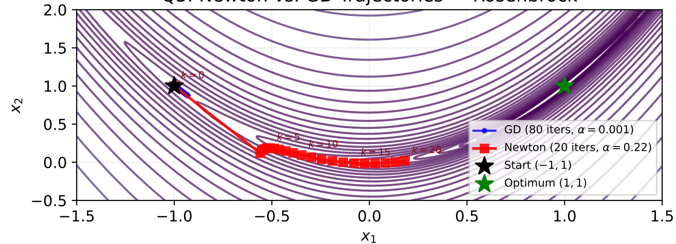
Q3: Newton vs. GD Trajectories — Rosenbrock
