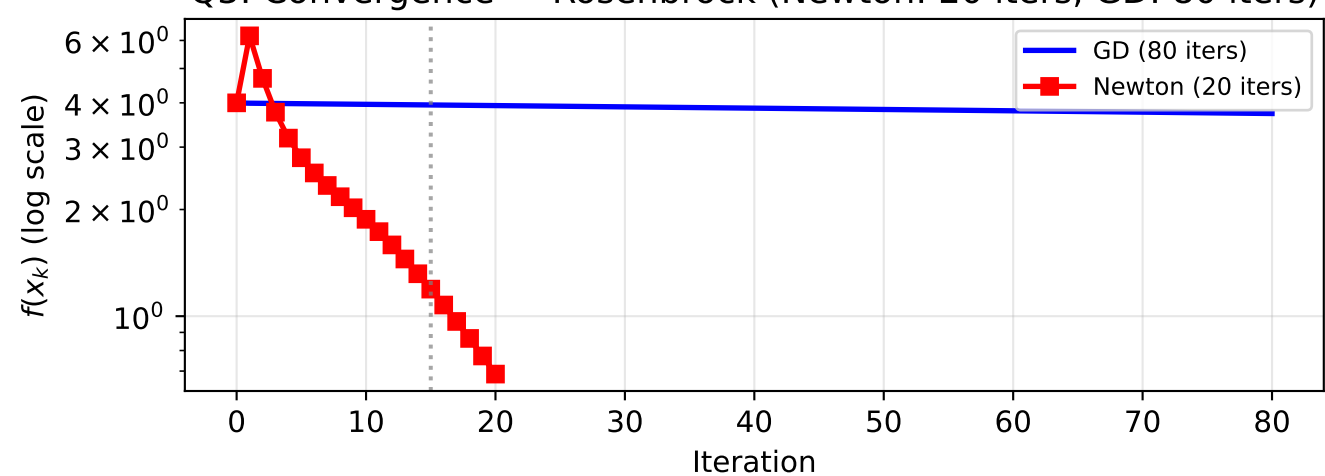
Q3: Convergence — Rosenbrock (Newton: 20 iters, GD: 80 iters)
