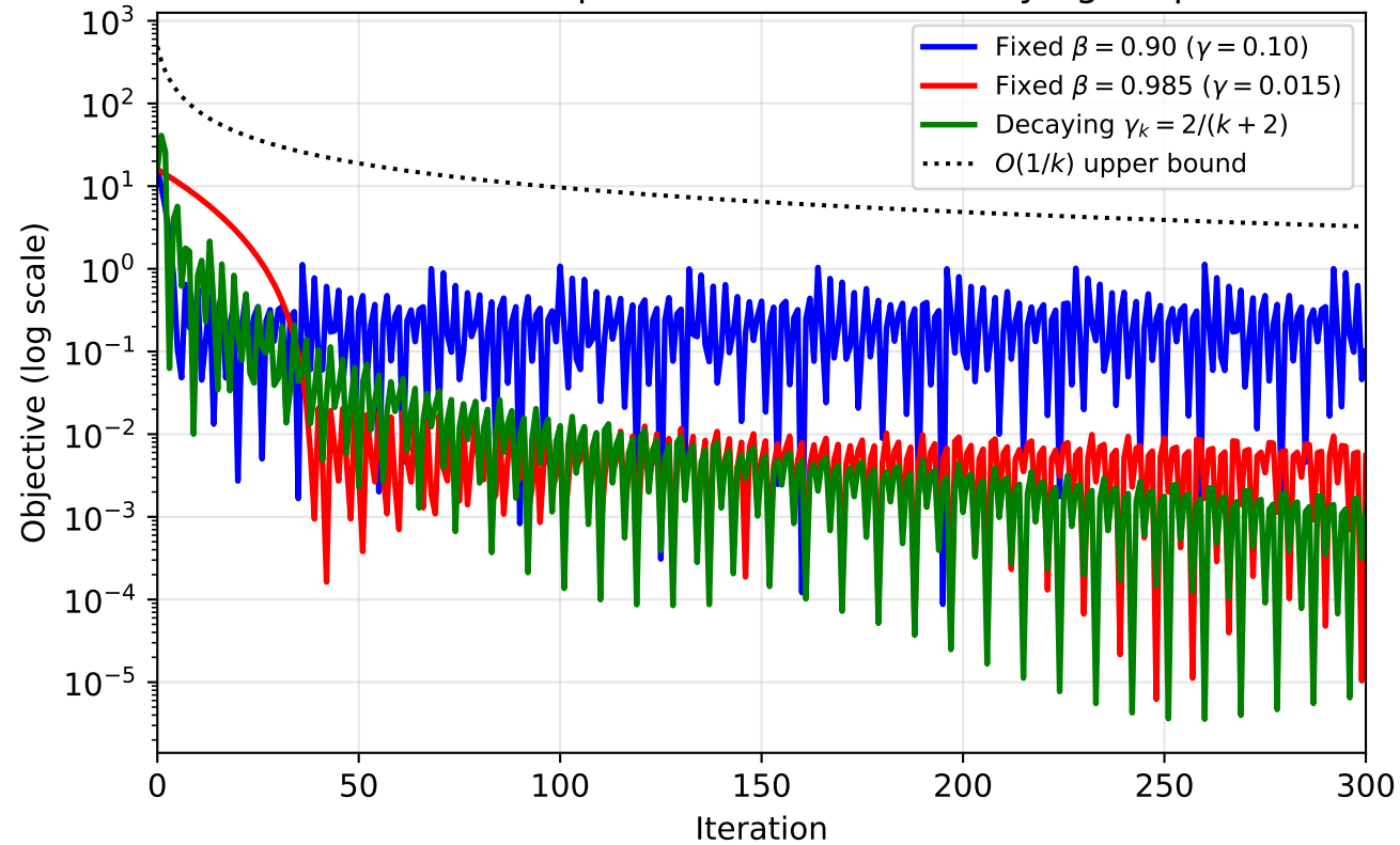
FW Interior Optimum: Fixed vs. Decaying Step
