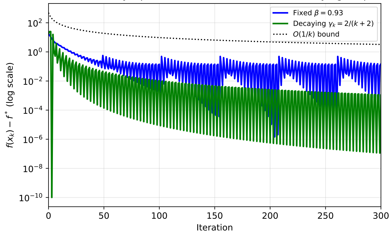
FW Boundary Optimum ( f^* = 0.25 ): Fixed vs. Decaying Step
