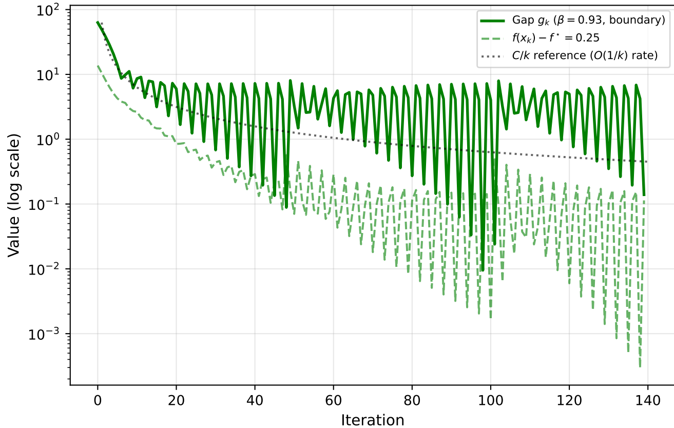
Q6: Frank--Wolfe Duality Gap (Boundary Case) with O(1/k) Reference
