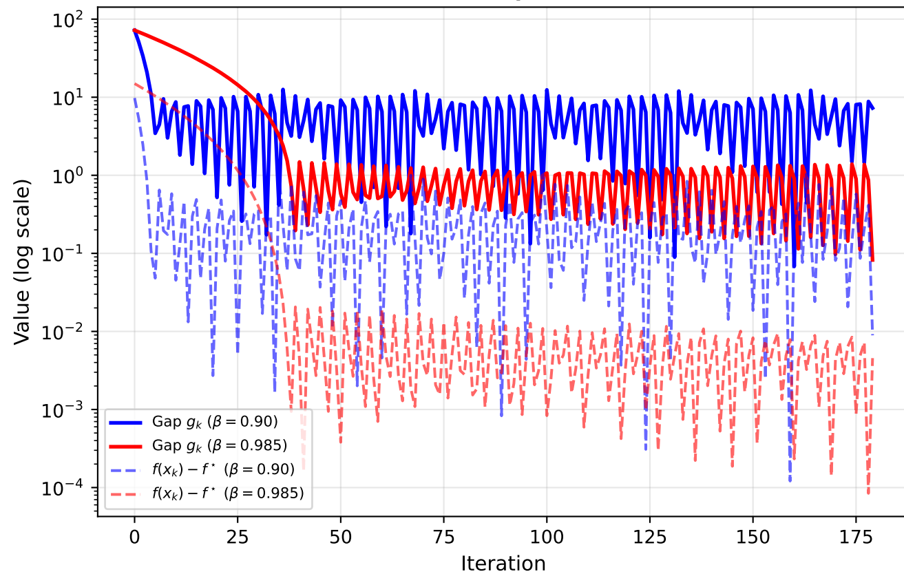
Q6: Frank--Wolfe Duality Gap vs Sub-Optimality (Interior Optimum)
