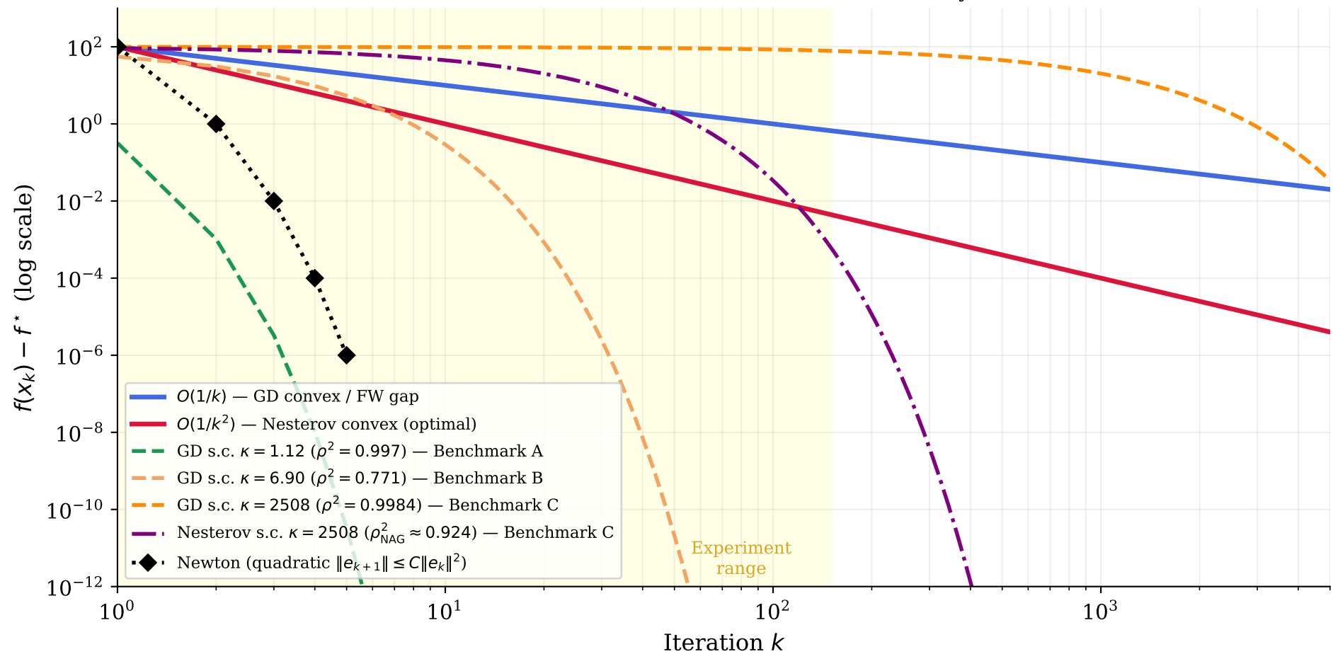
Theoretical Convergence Rates: All Benchmarks and Methods (Reference — Section 7 cross-method summary)
