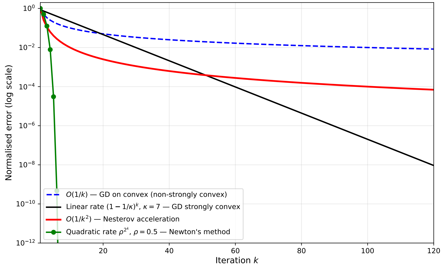
Theoretical Convergence Rate Comparison GD O(1/k) vs Nesterov O(1/k^2) vs Linear vs Newton Quadratic
